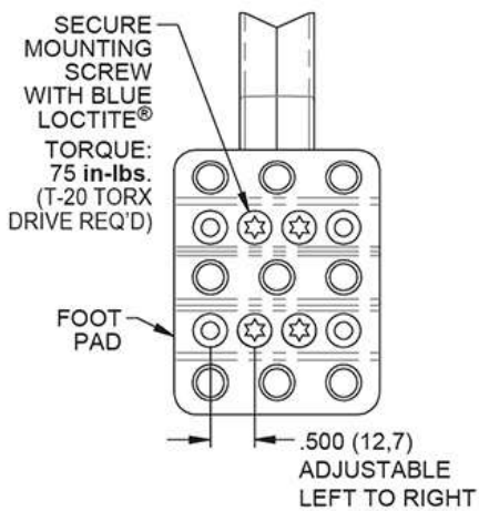
FOOT PAD DETAIL
